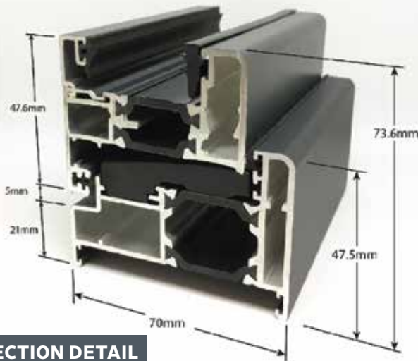
CONCEALED TRICKLE VENTILATION OPTION
